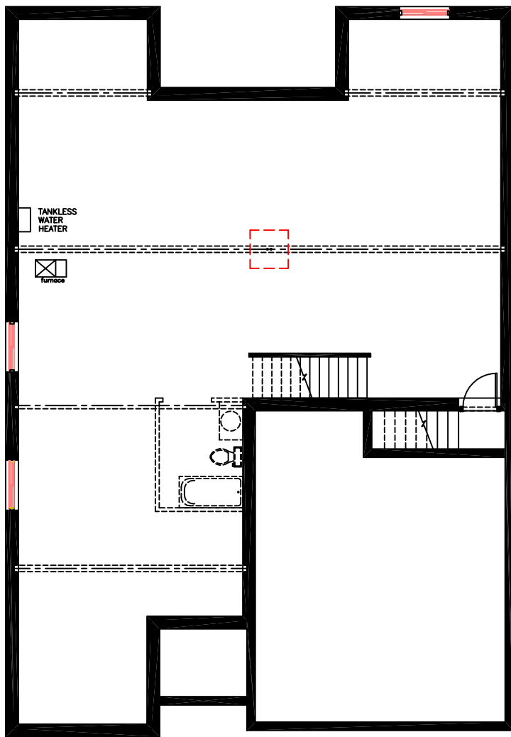
Basement level
