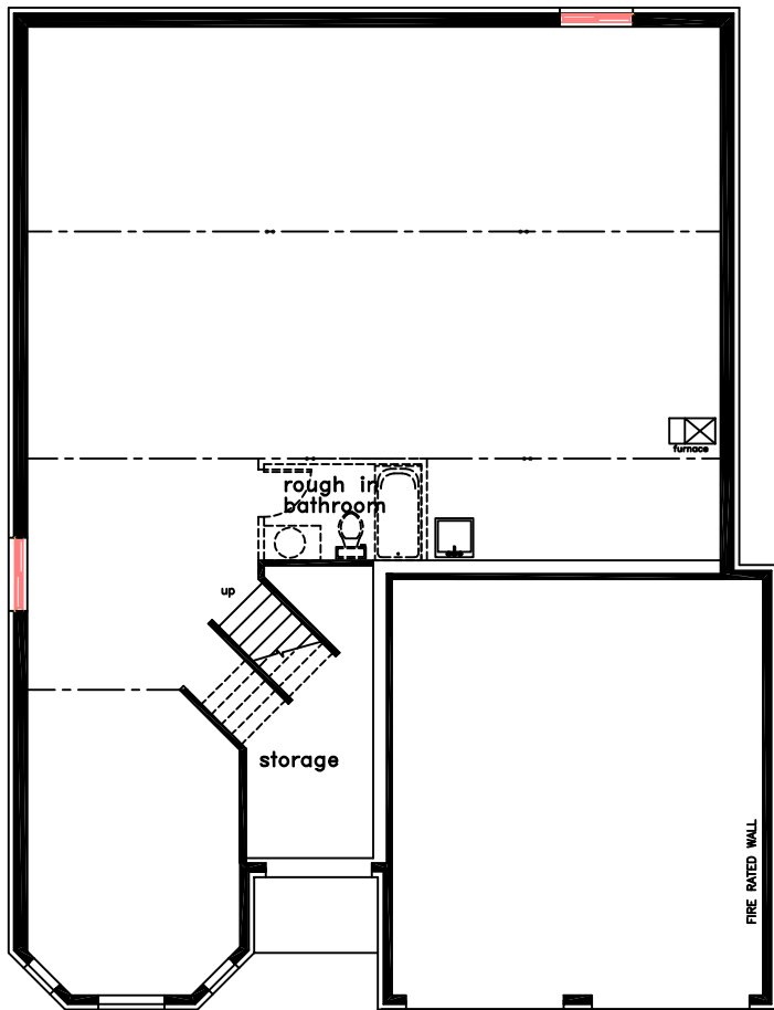
basement
